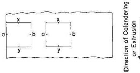
Points a , b and x , y are reference marks at midpoint of test specimen edges. FIG. 1 Method of Cutting Test Specimens from Sample
